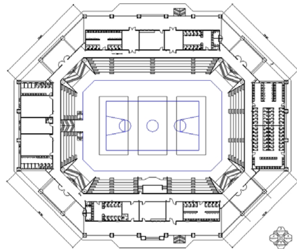
Plan of sports stadium.
